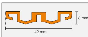
Schlüter®-KERDI-LINE-VARIO-WAVE 42 A
