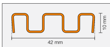
Schlüter®-KERDI-LINE-VARIO-WAVE-42 EB
