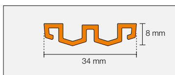
Schlüter®-KERDI-LINE-VARIO-WAVE 34 A
